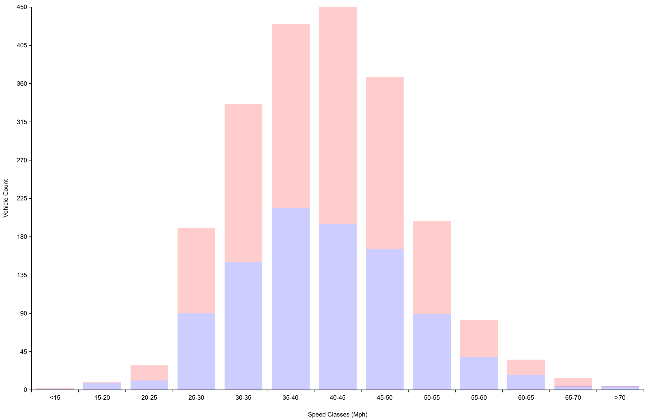
Vehicle Counts By Speed Class For week beginning Mon Nov 16 2020
