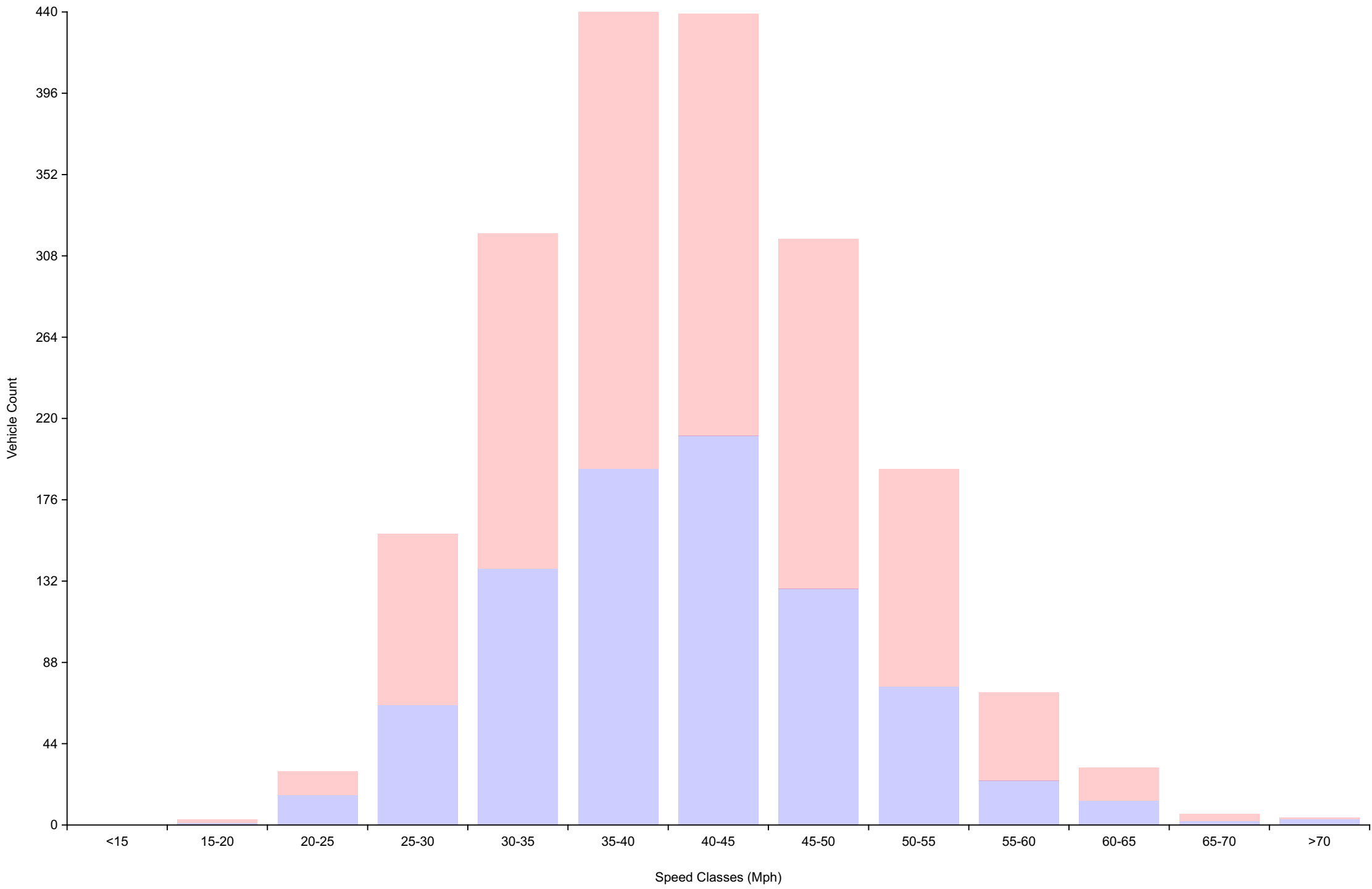
Vehicle Counts By Speed Class For week beginning Mon Nov 23 2020
