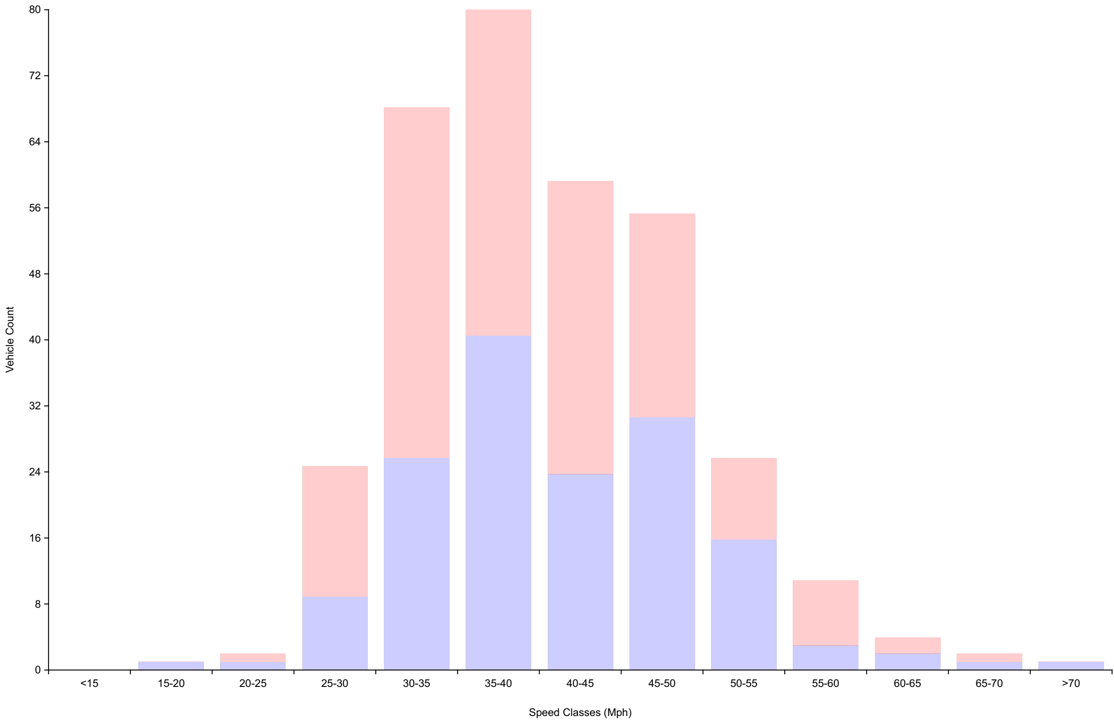
Vehicle Counts By Speed Class For week beginning Mon Nov 30 2020
